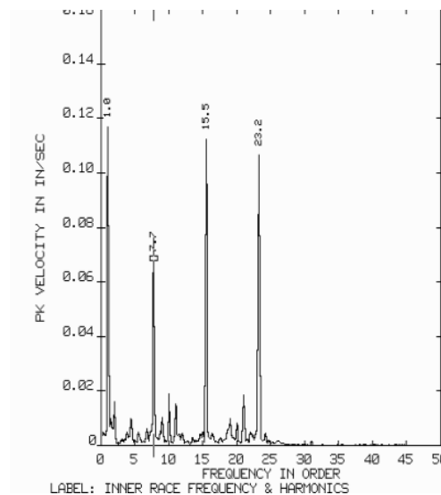
Figure 19: Spectrum plot showing a rolling element bearing with an inner race (BPFI) defect (Plot courtesy of Predictive Maintenance Services, Inc.)
