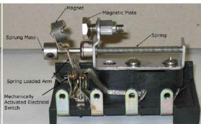
Fig. 6(b) Tripped mechanical switch mechanism with labeled parts
