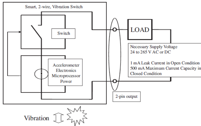
Figure 11 Typical connection schematic for a SMART Vibration Switch
