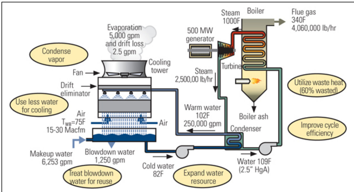
Figure 1. Cooling Tower process flow schematic
