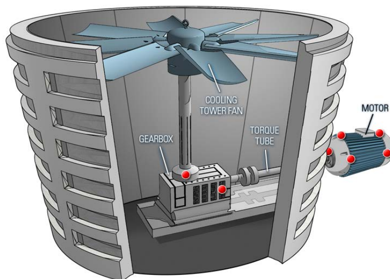
Figure 4. Cooling Tower components for an Industrial Cooling Tower
