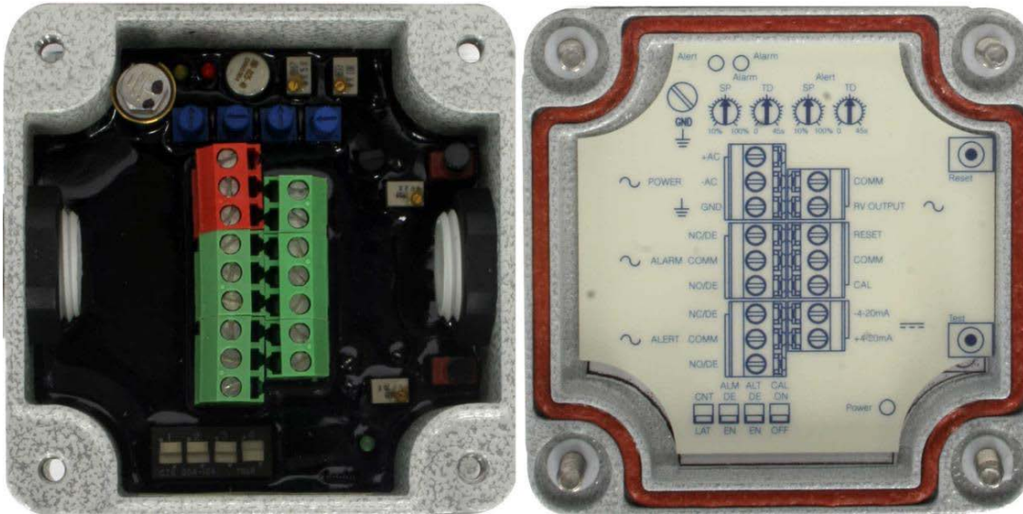
Figure 9 Electronic Vibration Switch internals
