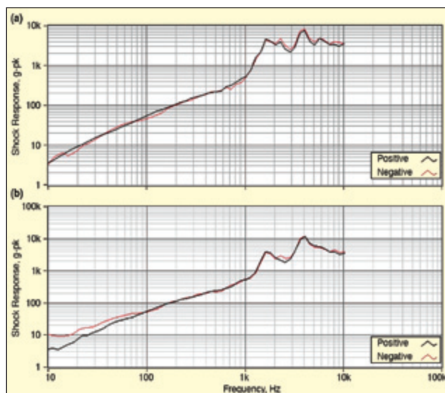
Figure 35: SRS data from tunable beam Test (a) 350C02; (b) 350B21.
