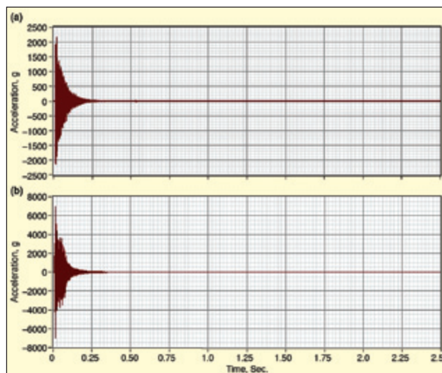
Figure 34. Acceleration data from tunable beam test; (a) 350C02; (b) 350B21.
