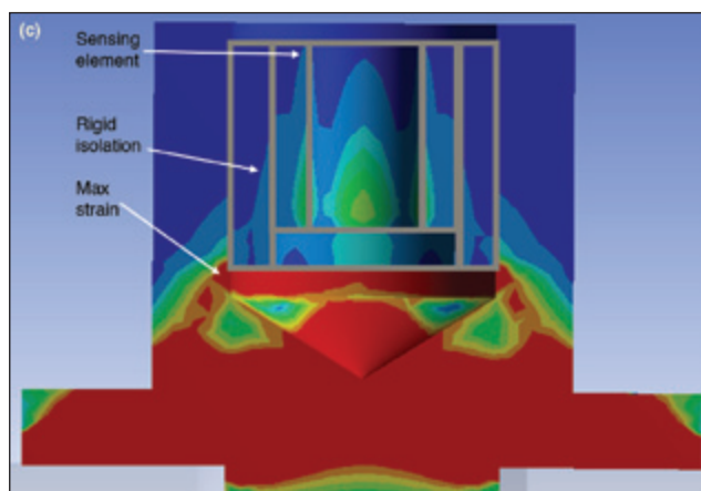
Figure 8. Effect of housing undercuts and rigid isolation on base strain: (a) standard housing, (b) undercut housing, (c) rigid, isolated housing.
